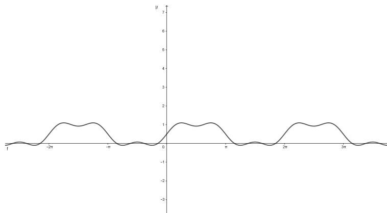
Figura 5.8: Soma parcial, S_3 = \frac{1}{2} + \frac{2}{\pi} \sin(x) + \frac{2}{3\pi} \sin(3\pi)
