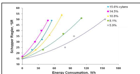
Figure 1. Effect of pulp xylan content on drainage resistance (°SR).
