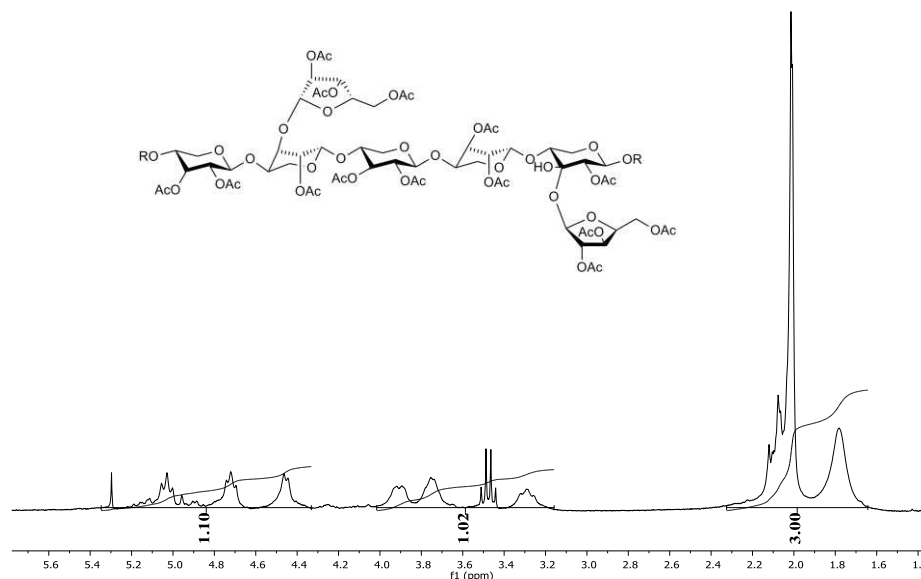
Figure 3. ^1\text{H} NMR spectrum acetylated hemicellulose (dissolved in \text{CDCl}_3 ) and structure of acetylated 4-O-methyl-(glucurono)arabinoxylans.
