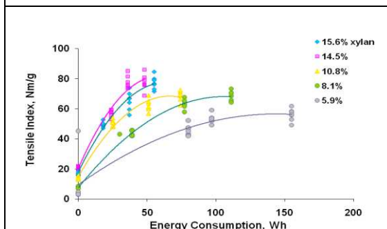
Figure 3. Effect of pulp xylan content on tensile index.
