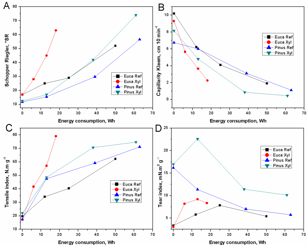
Figure 1. Effect of pulp xylan content on (A) drainage resistance (°SR), (B) capillarity Klemm, (C) tensile index, (D) tear index.
