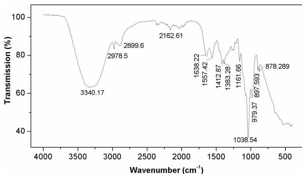
Figure 2. FT-IR spectra unmodified hemicelluloses.
