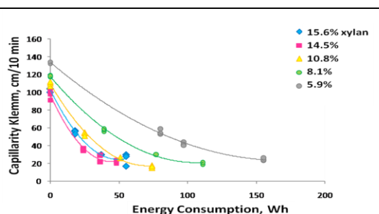
Figure 2. Effect of pulp xylan content on capillarity Klemm.
