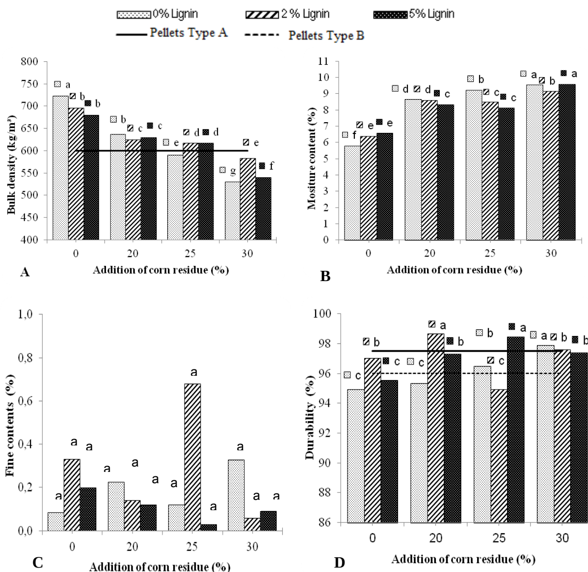
Figure 1. Properties of pellets for the treatments: A - Bulk density (kg m -3 ); B – Moisture content (%); C - Fine content (%); D - Durability (%). Bars followed by the same small letter don't differ among themselves at 5% probability (Scott, p > 0.05 ).
