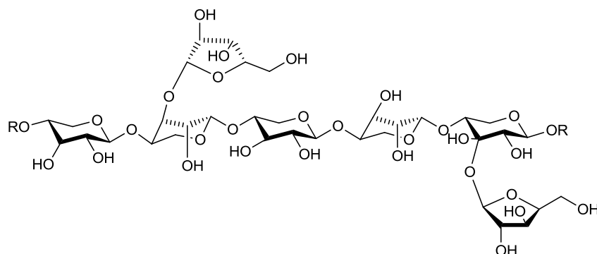
Figure 1. Typical xylan structure from corn fibers: 4-O-methyl-(glucurono)arabinoxylans.
