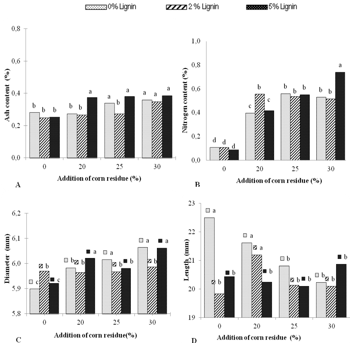
Figure 2. Properties of pellets for the treatments: A - Ash content (%); B – Nitrogen content (%); C - Diameter (mm); D - Mean length of the pellets (mm). Bars followed by the same small letter don't differ among themselves at 5% probability (Scott, p > 0.05 ).
