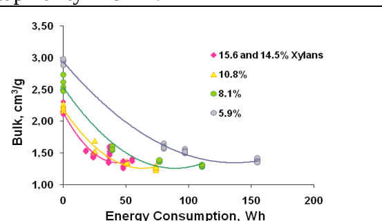
Figure 4. Effect of pulp xylan content on bulk.
