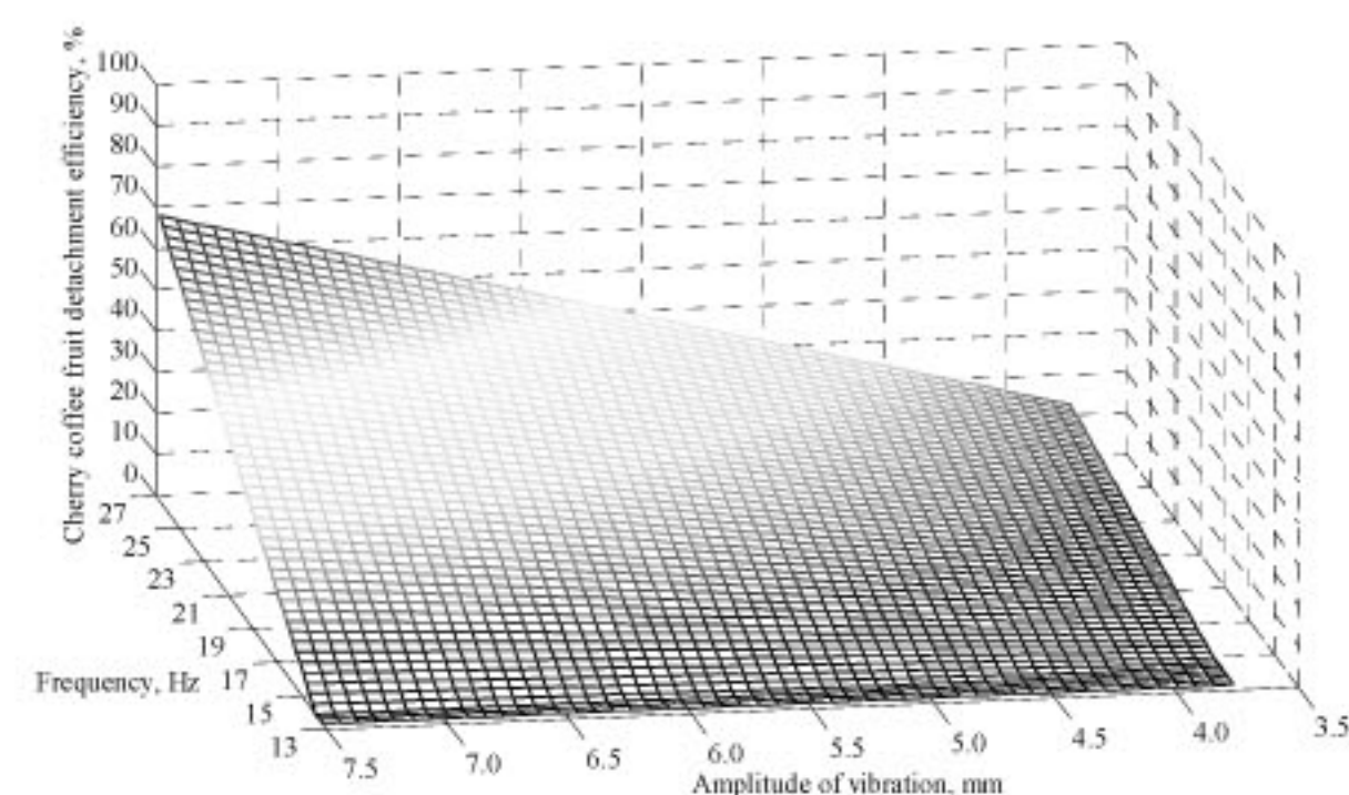
Figure 4. Response surface for the Catuaí Vermelho variety.
