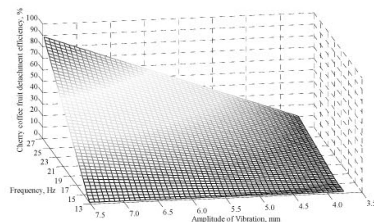
Figure 5. Response surface for the Mundo Novo variety.
