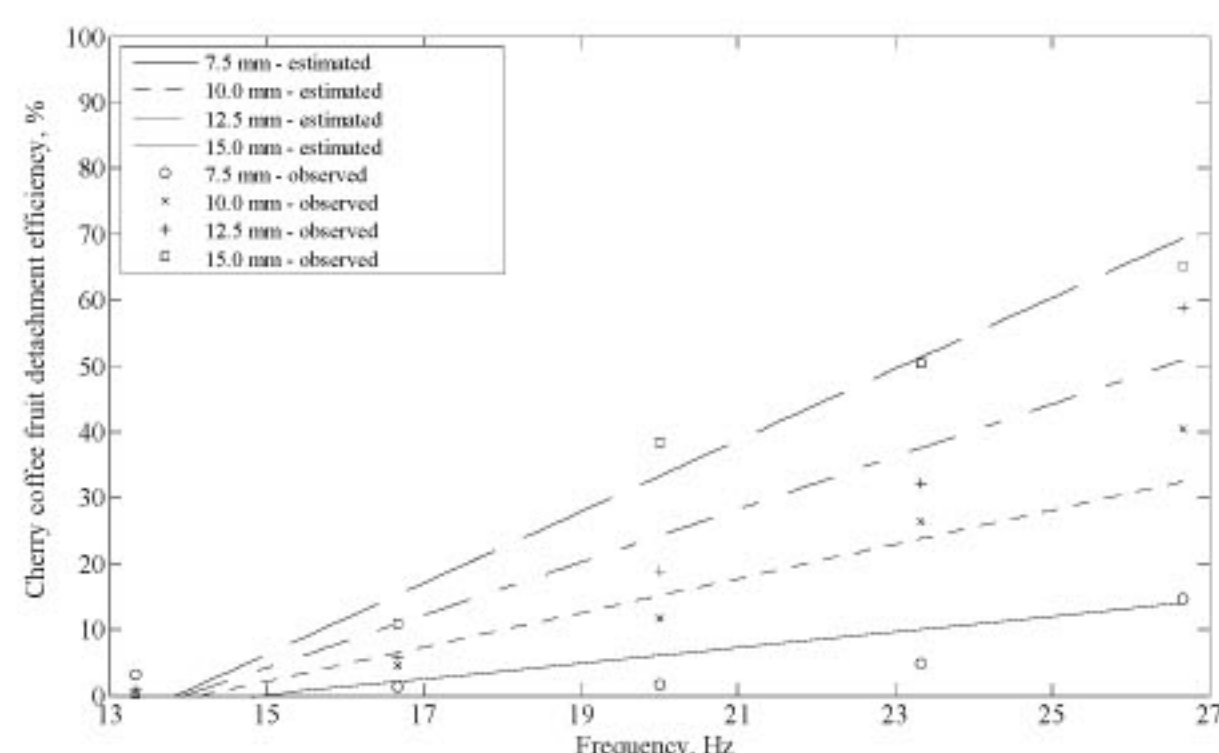
Figure 6. Response surface for cherry coffee fruit detachment efficiency generated at different vibration amplitude levels for different values of frequency for the Catuaí Vermelho variety.
