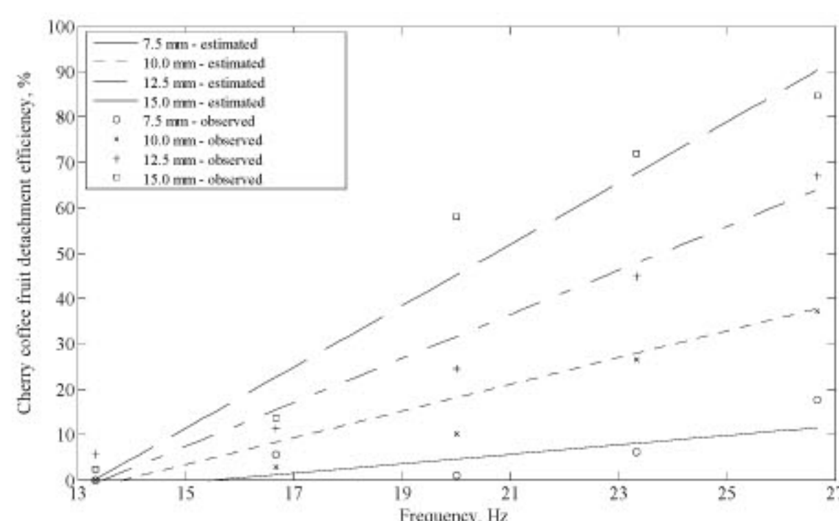
Figure 7. Response surface for cherry coffee fruit detachment efficiency generated at different vibration amplitude levels for different values of frequency for the Mundo Novo variety.
