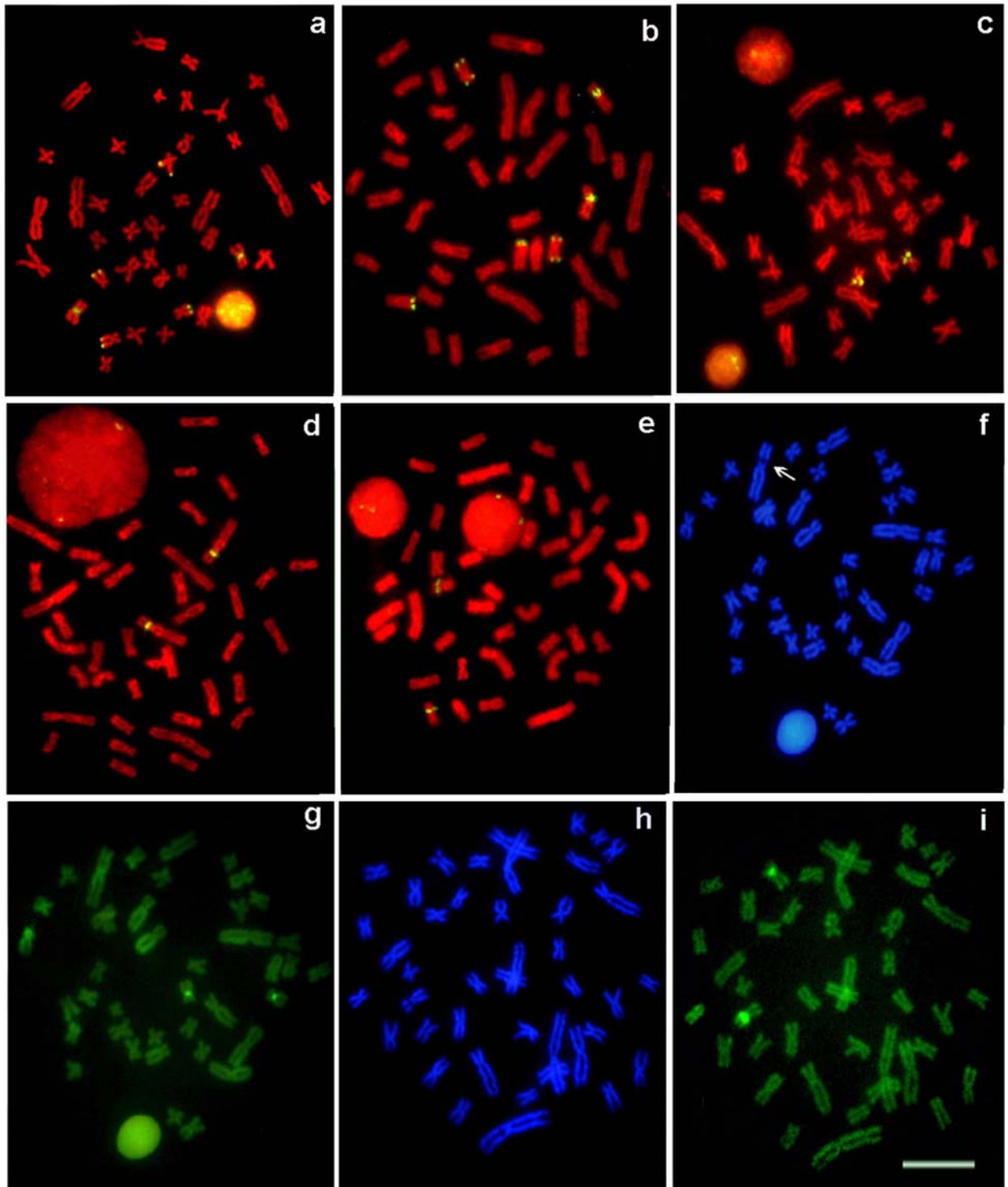
FIG. 3. Metaphase chromosome spreads of Hoplias malabaricus after FISH with 18S and 5S rDNA probes and DAPI/Chromomycin A3 staining. Numerical and positional variation of 18S rDNA sites in populations from (a) Pandeiros and Pará rivers, (b) Tombadouro Creek and Jacaré River. Mapping of 5S rDNA sites for populations of (c) Pandeiros and Pará rivers,
