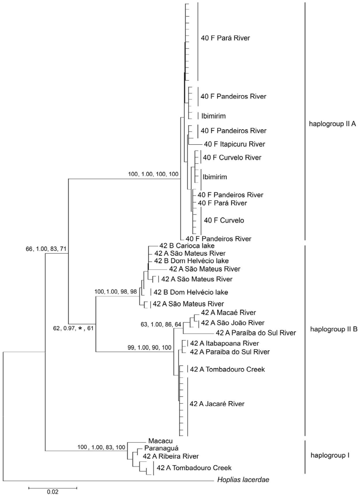
FIG. 6. Phylogenetic relationships of ATPase 6 haplotypes derived from H. malabaricus karyomorphs. The topology was obtained with neighbour joining
