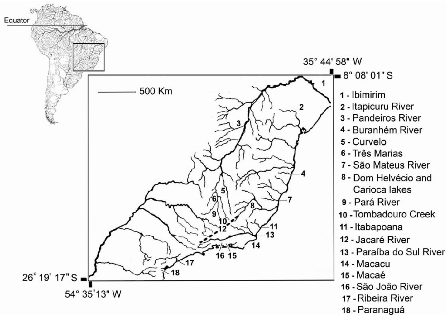
FIG. 1. Collection localities. The dotted line indicates the Upper Grande Crustal Discontinuity. The locality of Três Marias and Buranhém River are also depicted.
