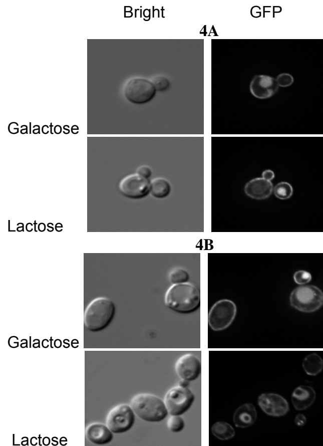
Figure 4 – Subcellular localization of LAC12GFPp when the JA6LAC12GFP strain was grown SC medium containing galactose or lactose as carbon source. 4A- After 2 hours of growth 4B- Overnight growth, The Lac12GFPp localization was analysed by fluorescence microscopy (Zeiss Axioplan2e microscope equipped with a 6100 alpha-Plan Fluor objective and differential-interference-contrast).
