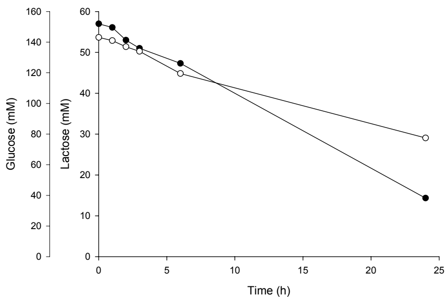
Figure 1 – Lactose and glucose consumption: The JA6LAC12GFP strain was grown on SC medium containing glucose 2% w/v ( 142,11 \text{ mmol}\cdot\text{L}^{-1} ) (○) plus lactose 2% w/v ( 58,48 \text{ mmol}\cdot\text{L}^{-1} ) (●).
