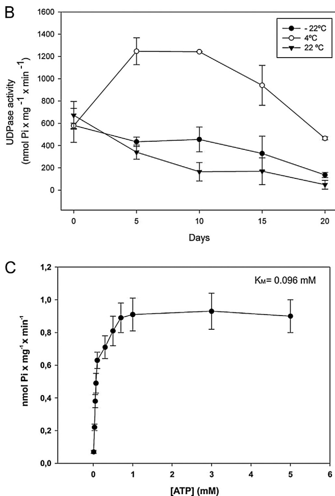
Fig. 1. Heterologous TcNTPDase-1 substrate specificity, stability and K_m . Enzyme activity was assayed using the malachite green method in a reaction buffer containing 50 mM HEPES, 50 mM Tris, 116 mM NaCl, 5.4 mM KCl, 2.5 mM MgCl 2 and 2.5 mM substrate, with the pH adjusted to 8.0. The results are the means ± SD from at least three independent experiments. After TcNTPDase-1 purification, each of the three samples was aliquoted and stored to verify the ideal storage temperature. Activity assays were performed for 20 days using UDP as a substrate (B). (C) The K_m for ATP. Activity was determined by measuring the hydrolysis of [ \gamma - 32 P] ATP. The results are the means ± SD from at least three independent experiments.
