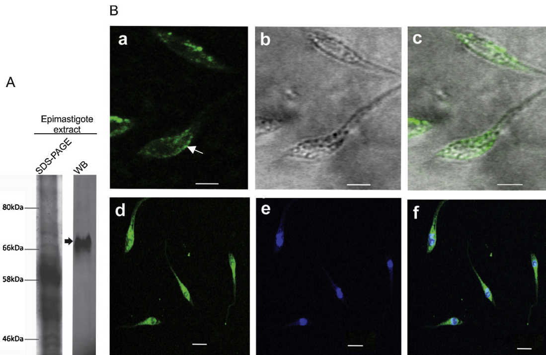
Fig. 2. Immunodetection of TcNTPDase-1 in T. cruzi . (A) Western blot (WB) analysis of TcNTPDase-1 expression in epimastigote extract. After incubation with rabbit antibodies anti-NTPDase-1 (1:1000) and anti-IgG conjugated with FITC (1:10,000), nitrocellulose membranes were analyzed in FLA 5100 (Fujifilm®). The SDS-PAGE gel was stained with Coomassie blue. (B) TcNTPDase-1 distribution in epimastigotes by confocal microscopy. Non-permeabilized parasites were fixed and stained with anti-TcNTPDase-1 (1:50) and visualized with Alexa 488-conjugated goat anti-rabbit IgG (a, d) (white arrow indicates the inner middle body), phase contrast (b) and merged (c, f). Nuclei and kinetoplasts were labeled with DAPI (e). Bar = 5 \mu m.
