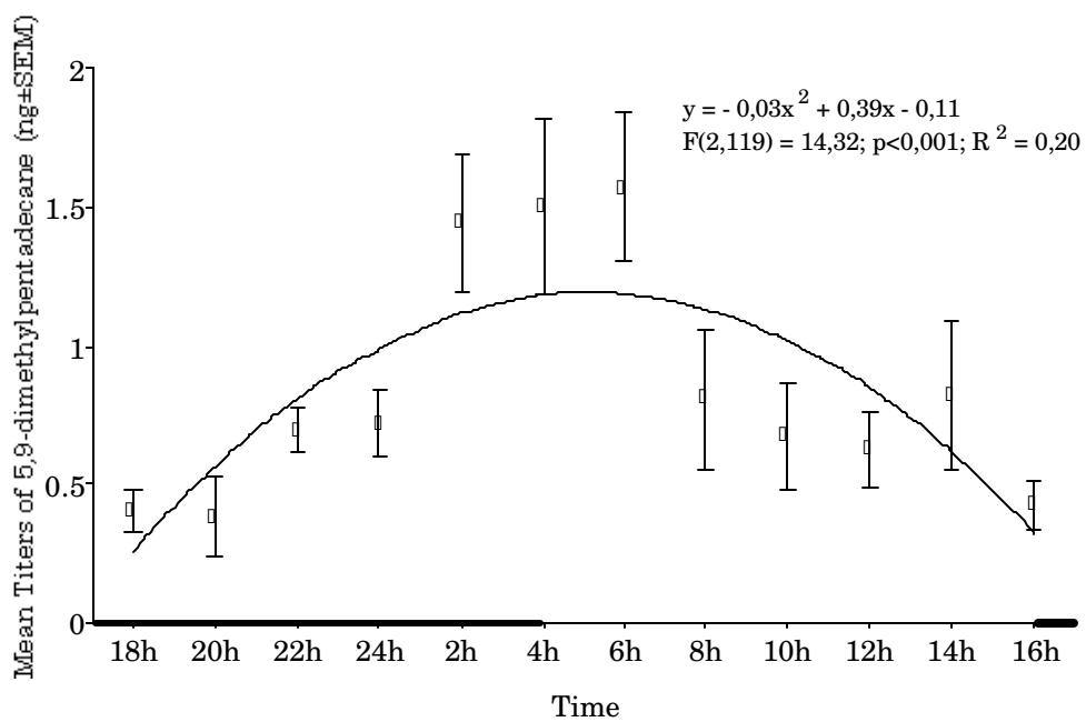
Figure 2 – Mean titers of the major compound, 5,9-dimethylpentadecane, extracted from two days old virgin females of Leucoptera coffeella . The scotophase is represented by the dark line on the time axis.
