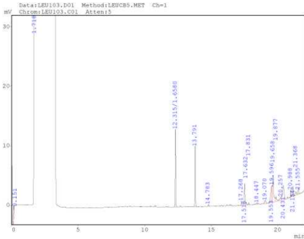
Figure 1 – Chromatogram of extract from virgin female of Leucoptera coffeella representing the retention times of the sex pheromone 5,9-dimethylpentadecane (12,315 min.) and the internal standard 5,9-dimethylhexadecane (13,791 min.).
