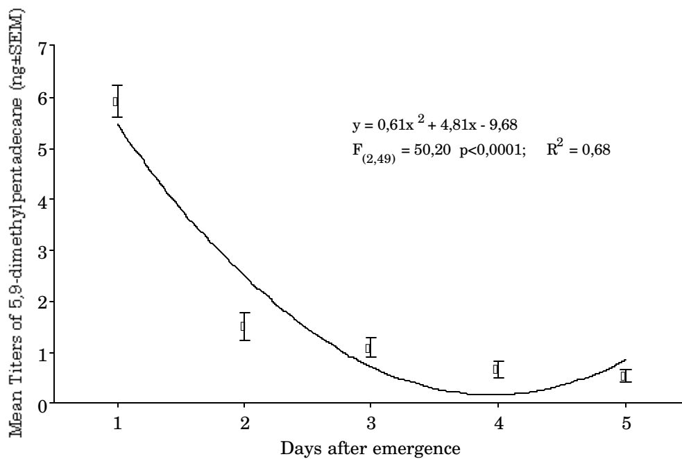
Figure 3 – Mean titers of the major compound, 5,9-dimethylpentadecane extracted from virgin females of Leucoptera coffeella from 1 to 5 days after emergence.
