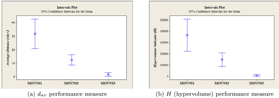
Fig. 4. Intervals plot
