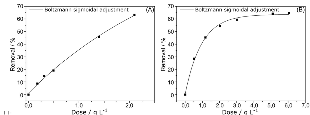
Figure 6S. Degradation of MO by nZVI of (a) Lot 01 and (b) Lot 02. Experimental conditions: C_0 (MO): 6 \times 10^{-5} \text{ mol L}^{-1} ; Volume of the solution = 50 mL and room temperature.
