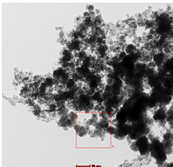
Figure 1S. Micrograph of nZVI by Transmission Electron Microscopy.
