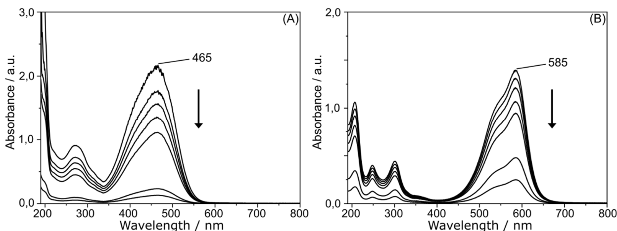
Figure 1. UV/Vis Molecular Absorption Spectra as a function of the concentration of (a) Methyl Orange and (b) Methyl Violet in solution at pH 5.5
