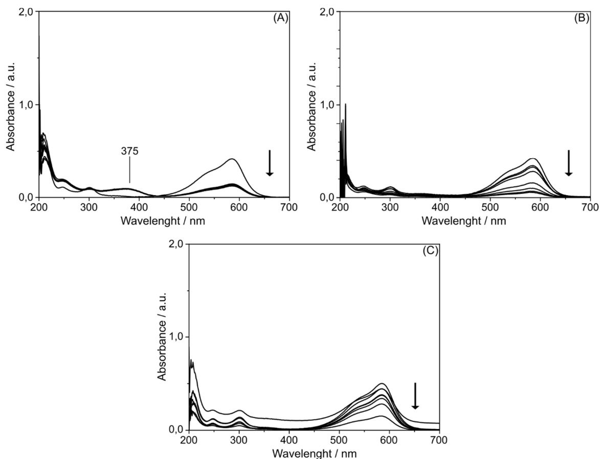
Figure 3S. UV / Vis Molecular Absorption Spectra of MO degradation as a function of time at (a) pH 2, variation between 0 and 3,5 minutes, (b) pH 4, variation between 0 and 16 minutes and (c) free pH, variation between 0 and 6 minutes.
