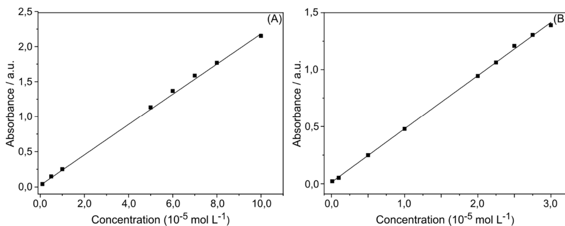
Figure 2. Analytical curves obtained from the UV/Vis Molecular Absorption Spectrophotometry analysis: (a) Methyl Orange (b) Methyl Violet. Experimental conditions: pH = 5, room temperature ( \sim 25^\circ \text{C} ), buffered system ( 0.1 \text{ mol L}^{-1} acetate buffer).
