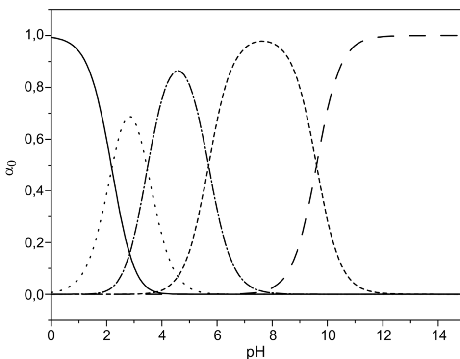
Figure 2S. Distribution of species of iron III complexes as a function of pH. Graph generated with the TitGer spreadsheet, where “———” represent the species \text{Fe}^{3+} , “·····” the ion \text{FeOH}^{2+} , “-----” the ion \text{Fe(OH)}_2^+ , “- · - · - ·” the ion \text{Fe(OH)}_4^- and “- - -” the ion \text{Fe(OH)}_3 .
