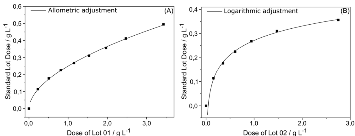
Figure 8. Adjustment between the nZVI dose from the standard lot (SL) with that from: (a) Lot 1 (L1) and (b) Lot 2 (L2). Experimental conditions: C 0 (MO): 6.00 \times 10^{-5} mol L -1 ; Volume of the solution = 50 mL; Room temperature (~25 °C).
