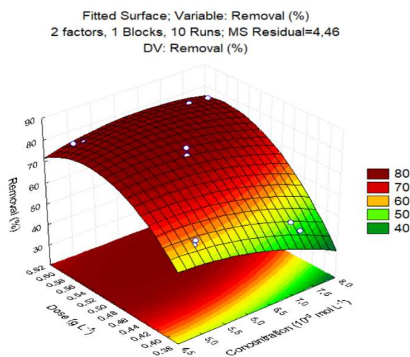
Figure 6. Response surface obtained from the factorial planning. Independent variables: nZVI dose ( \text{g L}^{-1} ) and MO initial concentration ( \text{mol L}^{-1} ), dependent variable (response): MO removal efficiency (%).
