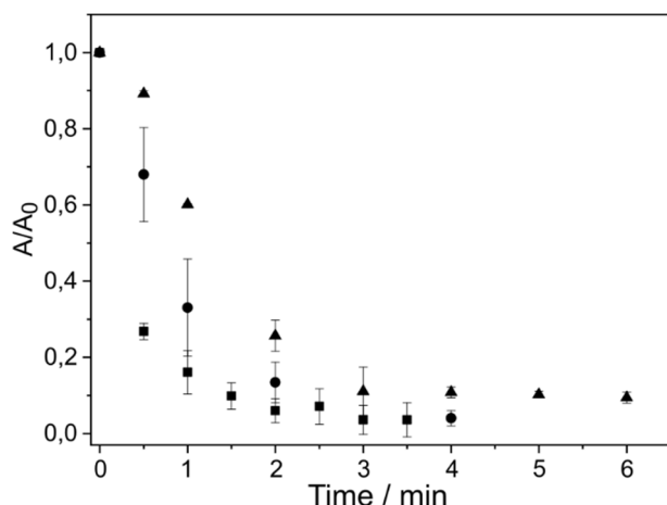
Figure 4. Removal efficiency of methyl orange. Experimental conditions: [MO]_0 = 6.00 \times 10^{-5} \text{ mol L}^{-1} ; nZVI dose = 0.5 \text{ g L}^{-1} (MO); V = 210 \text{ mL} ; Room temperature ( \sim 25^\circ \text{C} ); pH 2, 4 and without adjustment (pH0 of the dye solutions \sim 5.5 ); \blacktriangle pH without adjustment, \bullet pH 4; \blacksquare pH 2.
