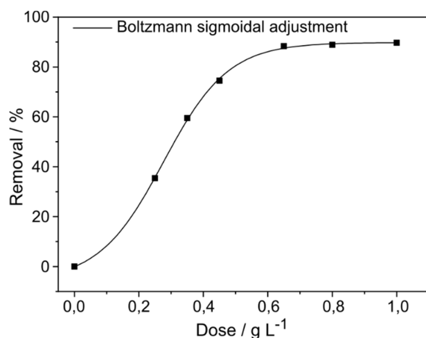
Figure 7. MO removal as a function of the nZVI (Standard Lot) dose.
