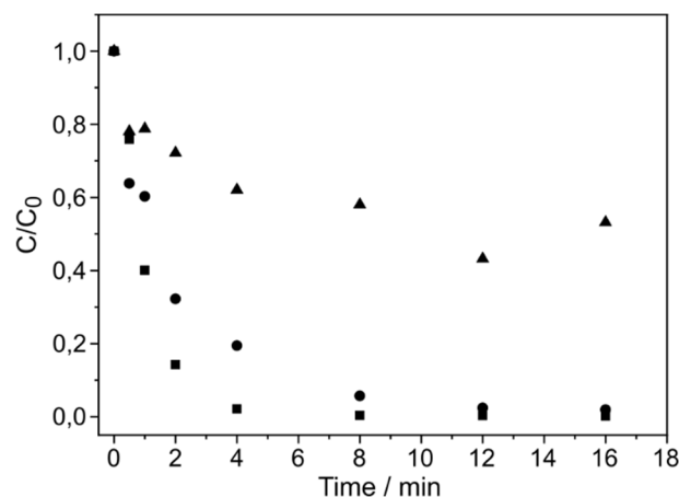
Figure 3. Dose study for dyes models. Experimental conditions: [MO] = 6 \times 10^{-5} mol L -1 , [MV] = 2.75 \times 10^{-5} mol L -1 ; nZVI doses = 0.5 g L -1 , 0.2 and 0.3 g L -1 ; V = 210 mL; room temperature (~25 °C); ▲ dose 0,2 g L -1 , ● dose 0,3 g L -1 , ■ dose 0,5 g L -1 .
