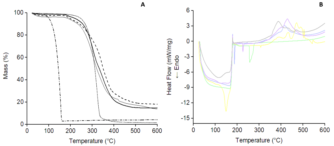
Figure 3. Thermogravimetric (TG) curves of lecithin (---) cholesterol (·····) carvacrol (-·-·-) carvacrol-loaded liposomes suspension (—) and empty liposomes suspension (—) (A). Differential scanning calorimetry (DSC) curves of lecithin (blue curve) cholesterol (yellow curve) carvacrol (green curve) carvacrol-loaded liposomes suspension (purple curve) and empty liposomes suspension (gray curve) (B).
