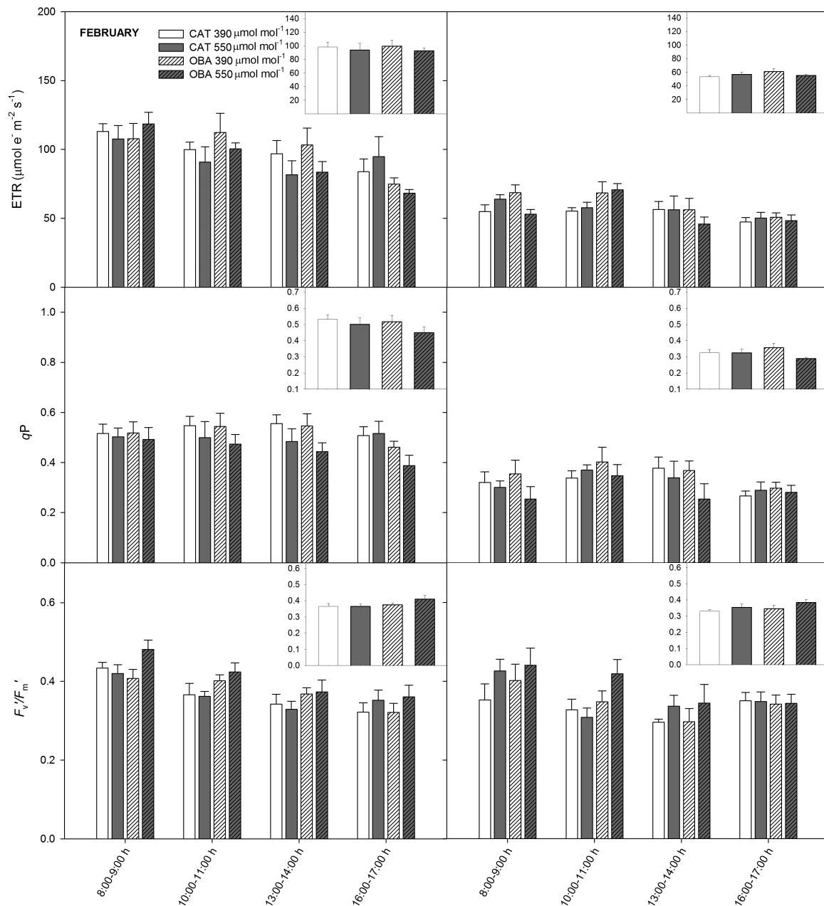
Fig. 2. Effect of elevated ( 550 \mu\text{mol mol}^{-1} ) and ambient ( 390 \mu\text{mol mol}^{-1} ) [\text{CO}_2] on the photochemical parameters of two coffee cultivars (Catuaí and Obatã) growing in a FACE trial during the growing season (February) and winter (August): electron transport rate (ETR), photochemical quenching coefficient ( q_p ), and capture efficiency of excitation energy by open PSII reaction centres ( F_v'/F_m' ). In the insets, the mean diurnal values of ETR, q_p , and F_v'/F_m' are shown. The [\text{CO}_2] used during the chlorophyll a fluorescence measurements was identical to the growth [\text{CO}_2] . n=6 \pm \text{SE} .
