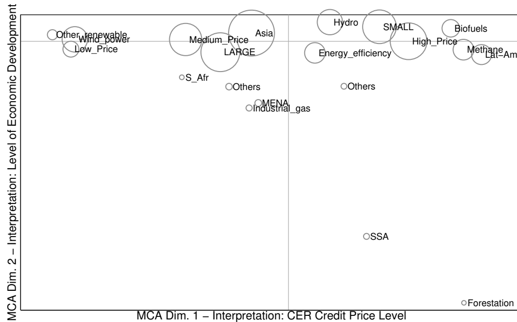
Figure 26 – Multiple Correspondence Analysis Biplot
