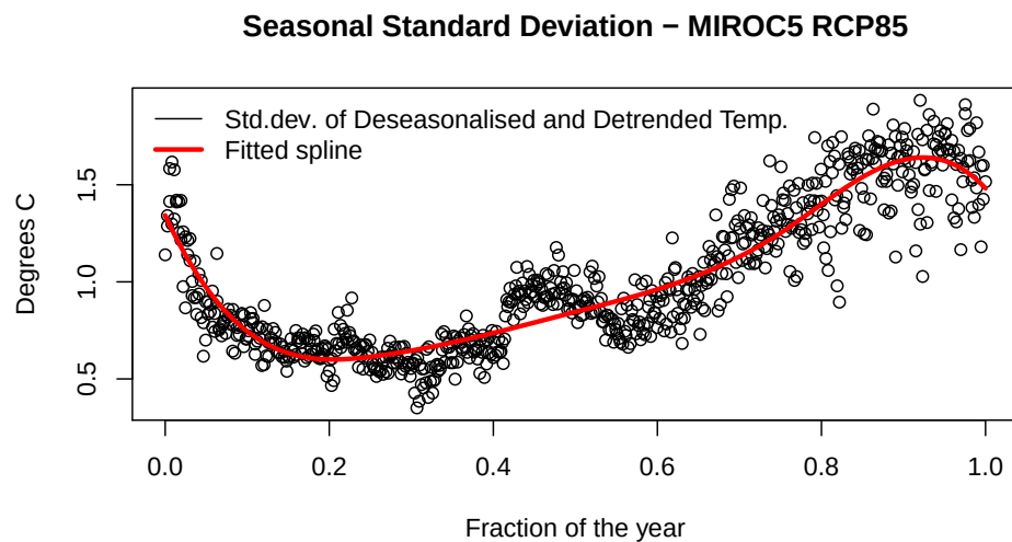
Figure 15 – Standard deviation of the detrended and deseasonalised maximum daily temperature from a single weather station (820980) throughout the year, and a spline fitted to the data.
