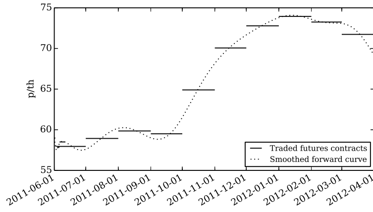
Figure 2 – Closing prices of UK Natural Gas futures contracts on June 1 2011, together with a smoothed price curve. Source: Authors' elaboration based on data from ( INTERCONTINENTAL EXCHANGE, 2012 ) and research results.
