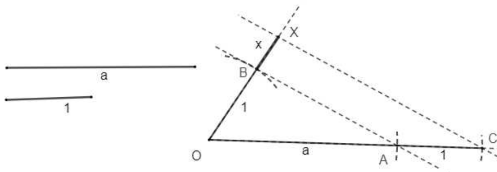
Figura 3.8: x = \frac{1}{a} .
