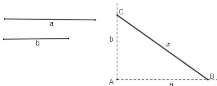
Figura 3.14: x = \sqrt{a^2 + b^2}
