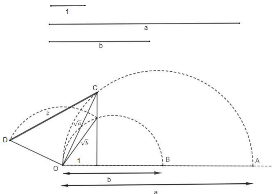
Figura 3.16: z = \sqrt{a + b}
