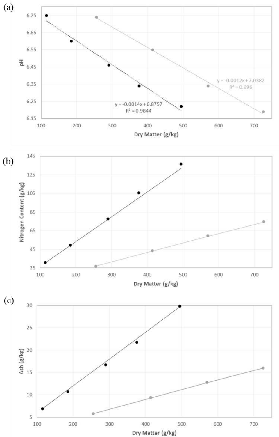
Figure 3 – Evolution of (a) pH, (b) total nitrogen and (c) ash contents of concentrates during concentration of non-sweetened (NSw) and sweetened (Sw) homogenized milks at pilot scale. Legend: Experimental data ( • ) NSw and ( • ) Sw; Theoretical data ( — ) NSw and ( — ) Sw; Tendency lines ( — ) NSw and ( — ) Sw.
