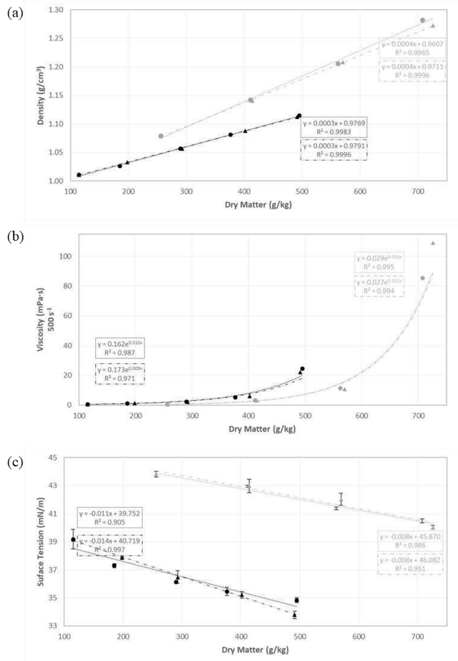
Figure 5 – Evolution of some physical properties of non-sweetened (black) and sweetened (gray) milk concentrates during concentration using a pilot scale evaporator (○) and a lab-scale evaporator (Δ): (a) density, (b) viscosity and (c) and surface tension.
