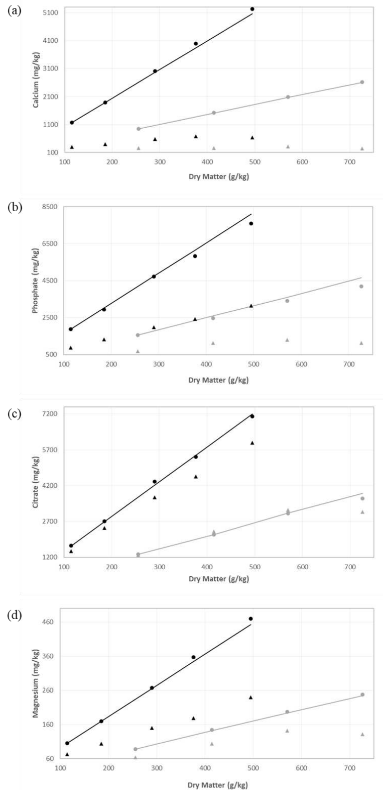
Figure 4 – Evolution of total and soluble ion contents during concentration of non-sweetened (NSw) and sweetened (Sw) homogenized milks: (a) calcium, (b) phosphate, (c) citrate and (d) magnesium. Legend: Theoretical Total (•) NSw and (•) Sw; Experimental Total (▲) NSw and (▲) Sw; Soluble Experimental (—) NSw and (---) Sw.
