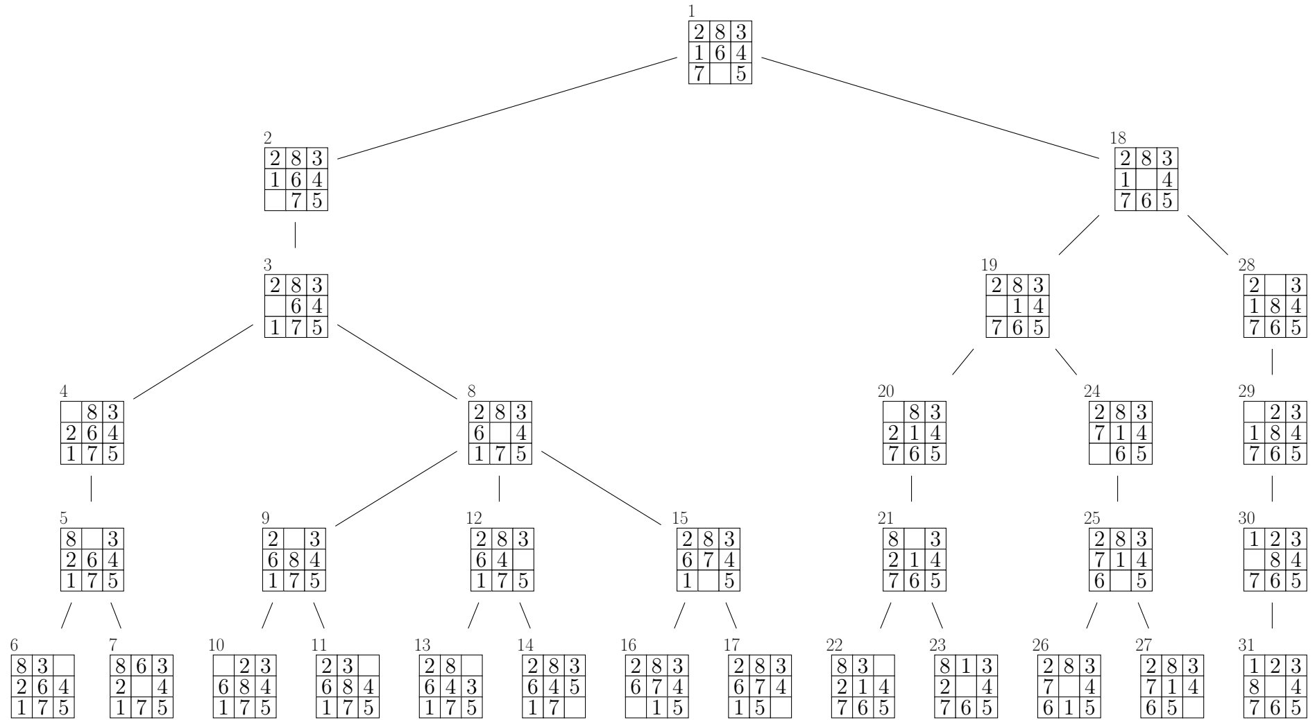
Figure 1 – 8 tile puzzle using DFS. (CHEN, 2011)
