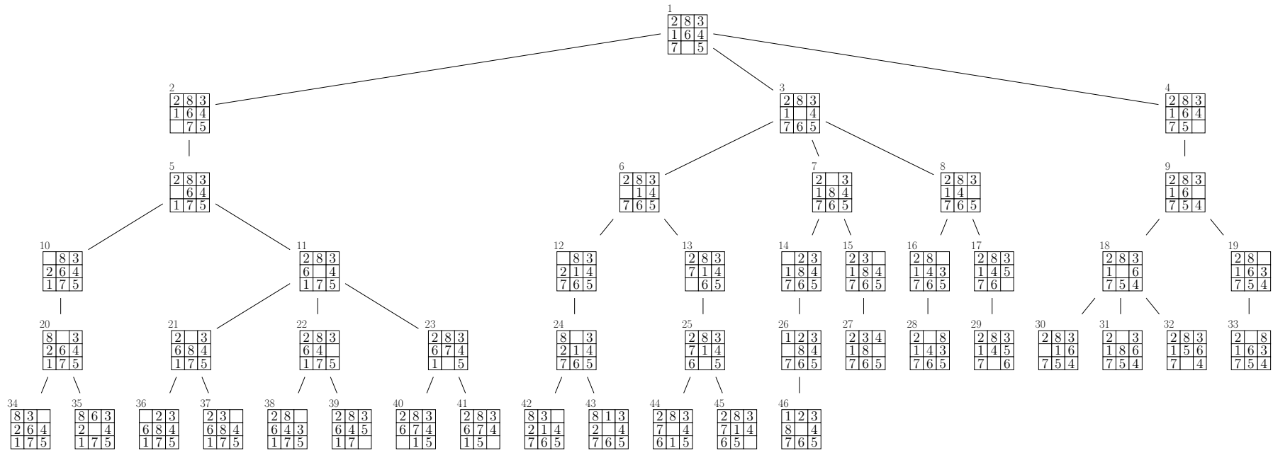
Figure 2 – 8 tile puzzle using BFS. (CHEN, 2011)
