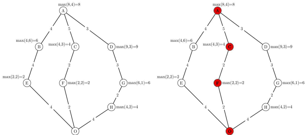
Figure 9 – The left figure shows a state space graph where the number above of each node is the maximum heuristic value of h_1 and h_2 . The initial state is A and the goal state is O. The right figure shows a state space where the highlighted states are those expanded by A*.
