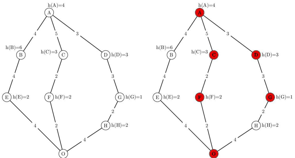
Figure 8 – The left figure shows a state space graph where the number above of each node is the heuristic value assigned by a heuristic h_2 . The initial state is A and the goal state is O. The right figure shows a state space where the highlighted states are those expanded by A*.
