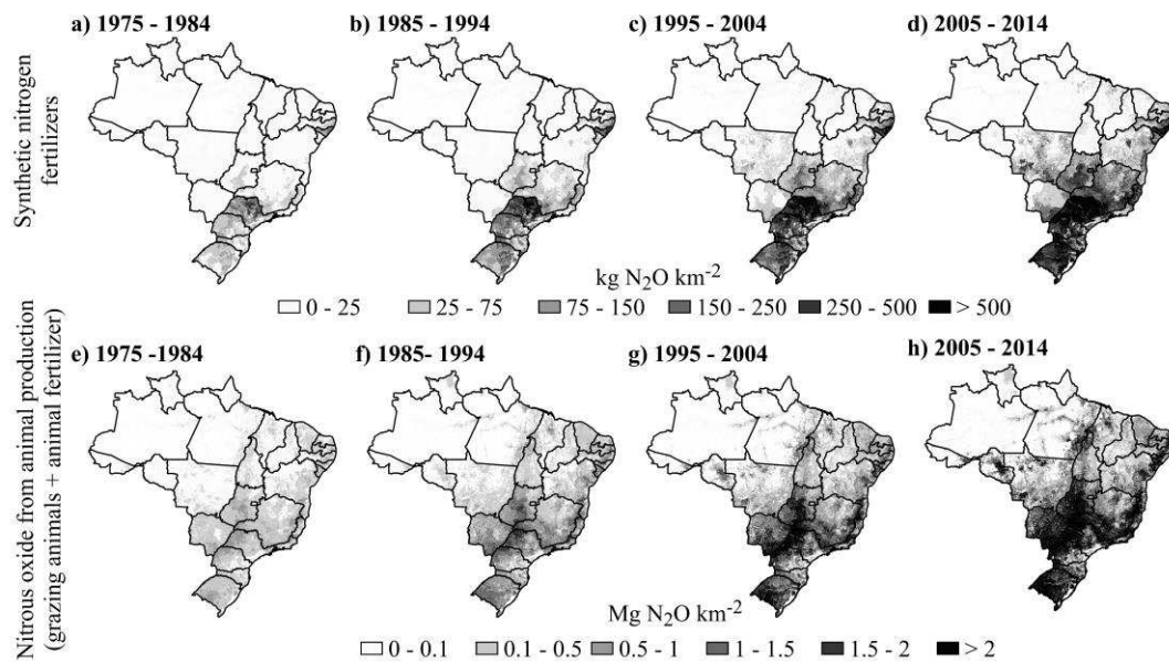
Fig. 2.7: The distribution and intensity of N_2O emissions from synthetic nitrogen fertilizers used in agriculture for the periods (a) 1975-1984, (b) 1985-1994, (c) 1995-2004, and (d) 2005-2014, and from grazing animals and manure used as fertilizers for the years of (e) 1975-1984, (f) 1985-1994, (g) 1995-2004, and (h) 2005-2014. The map data corresponds to the sum of the emissions during the period.
