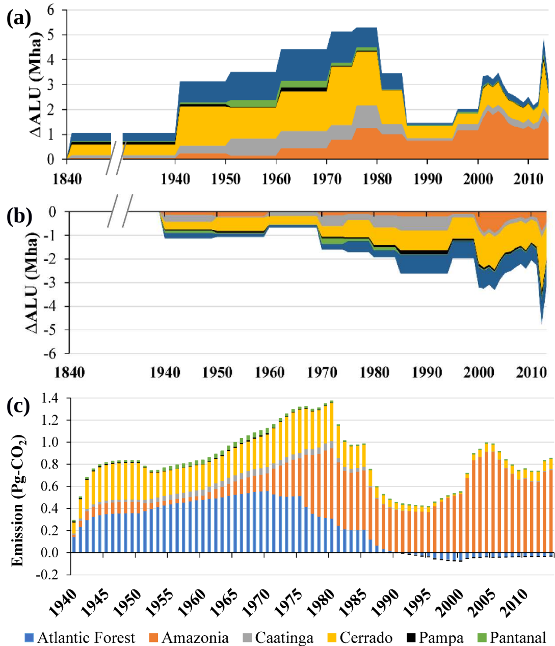
Fig. 2.4 Change in agricultural area results in (a) deforestation from agriculture expansion ( \Delta\text{ALU} > 0 ) in million hectares, (b) secondary vegetation grow from agriculture abandonment ( \Delta\text{ALU} < 0 ) in million hectares, and (c) CO 2 emission between 1940 and 2014 for each biome.
