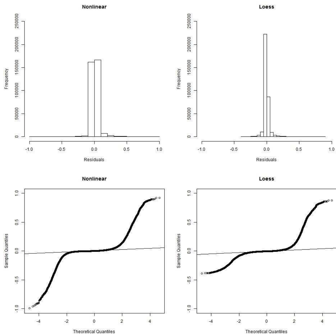
Figure S1. Residual frequency and QQ plot for nonlinear and loess regression in DL2.
