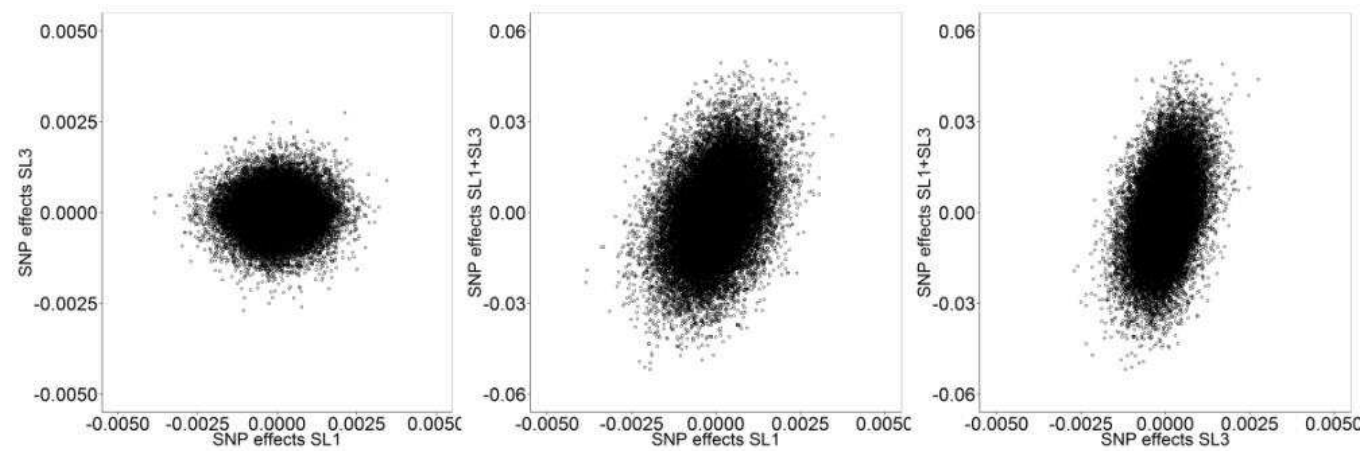
Figure 5.3 Dispersion plot for backfat thickness for SL1, SL3 and the combined data set (SL1+SL3).
