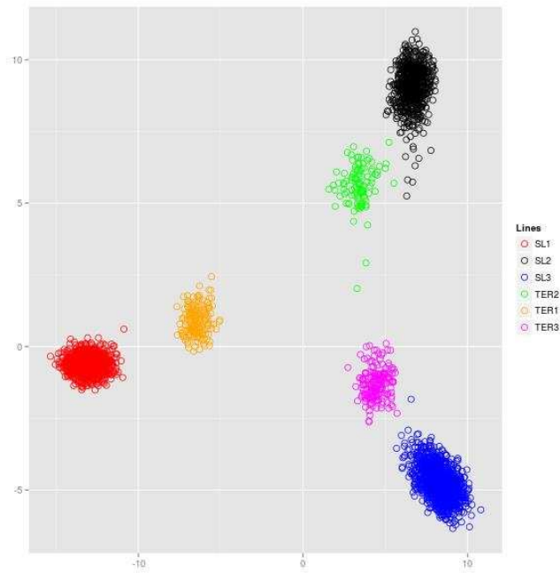
Figure 4.1 Multidimensional scaling showing a two dimensional projection of the populations distances.
