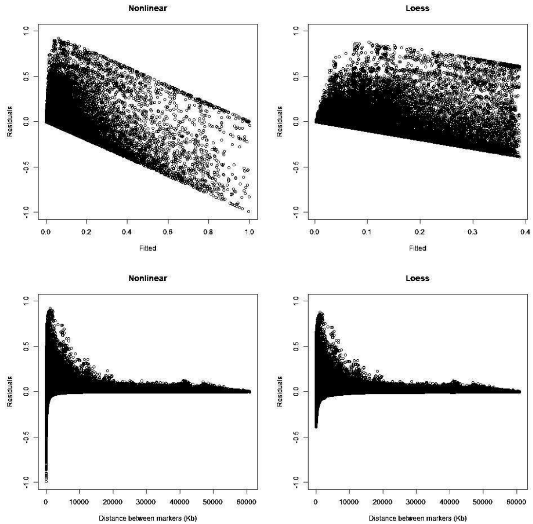
Figure S2. Plots of the residuals against fitted values (top) and against the distance between markers (bottom) for nonlinear (left) and loess regression (right) in line DL2.
