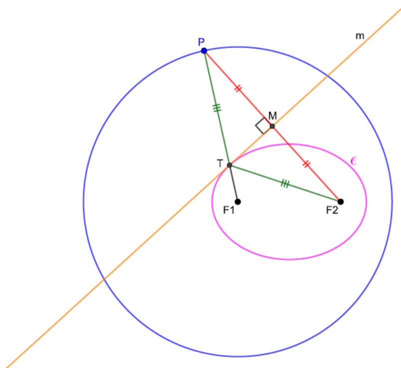
Figura 5.3: Elipse \epsilon com focos F_1 e F_2
