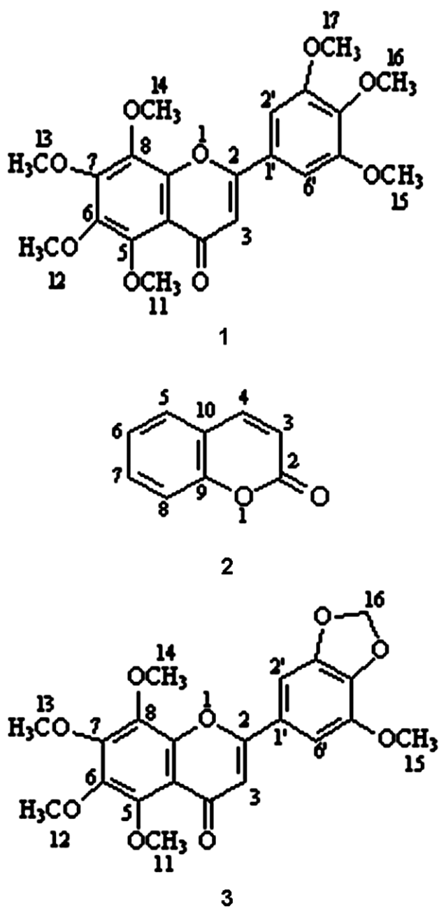
Figure 1. Structures of compounds isolated from A. conyzoides : 5,6,7,8,3',4',5'-heptamethoxyflavone (1), coumarin (2) and 5,6,7,8,3'-pentamethoxy-4',5'-methylenedioxyflavone (3).
