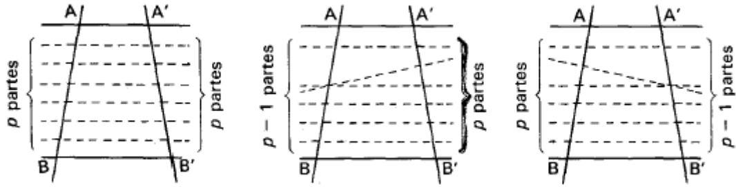
Figura 4.4: Tales-2, [29].
