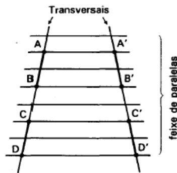
Figura 4.3: Tales-1, [29].
