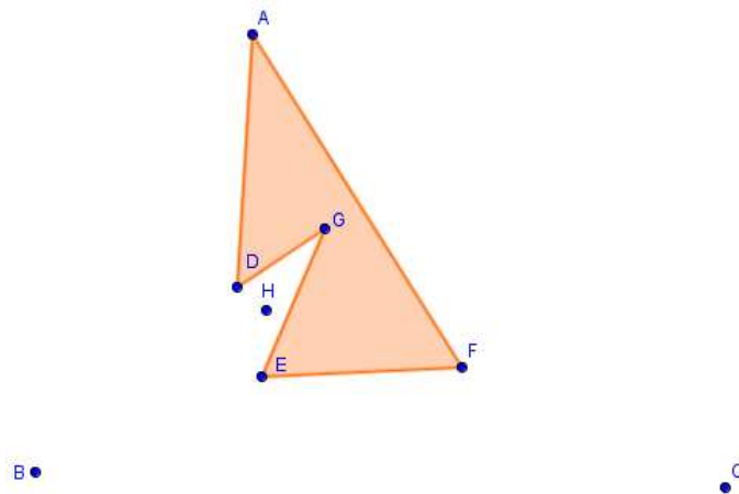
Figura 6.22: Pentágono ADGEF.
